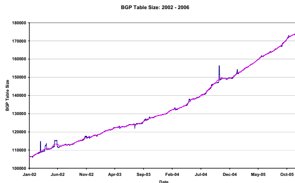
Figure 6. BGP Prefix Table Size
