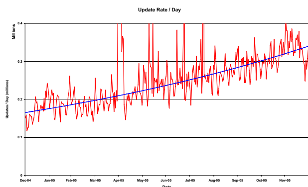
Figure 5. Prefix Withdrawal Counts
