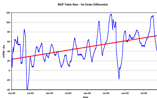
Figure 7. First order differential of BGP Table Size
