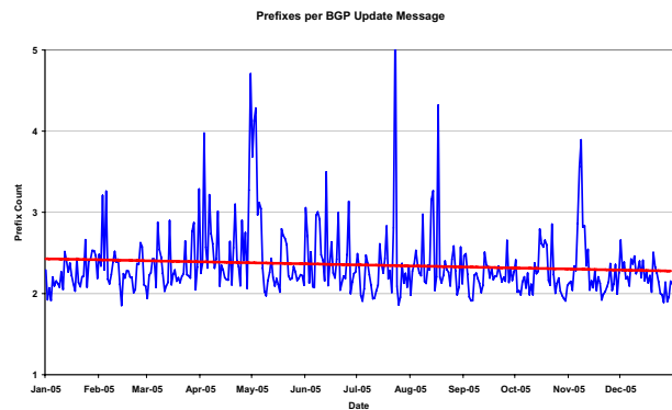
Figure 2. Average number of Prefixes per Update Message
