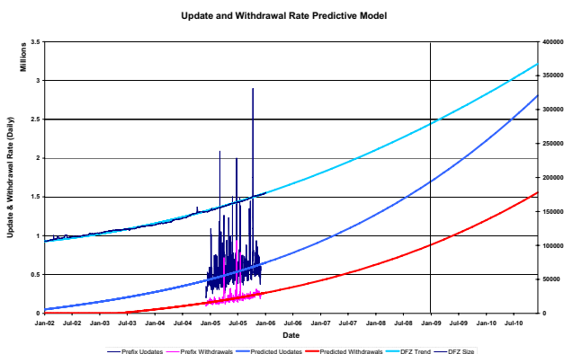
Figure 10. Prefix Update Rate Projection
