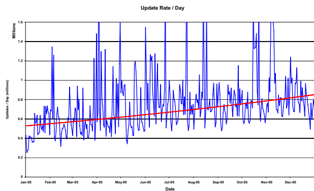
Figure 4. Prefix Update Counts
